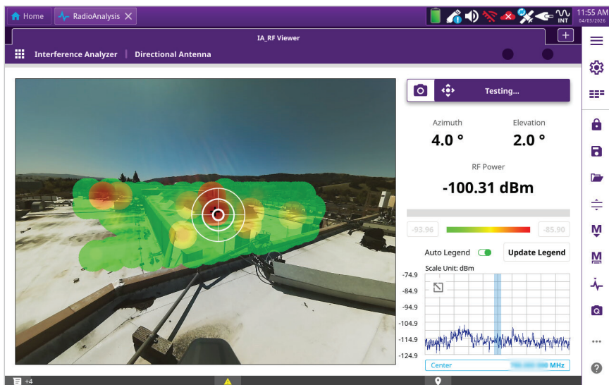
RF Viewer | PIM Generated Interference | Case 2 Sector Top NE
