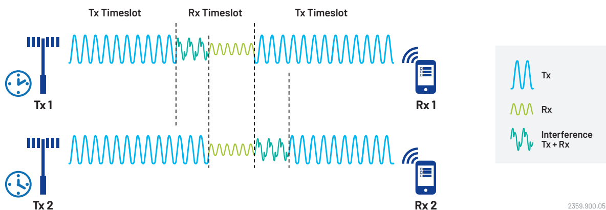
Synchronization and Interference in TDD
