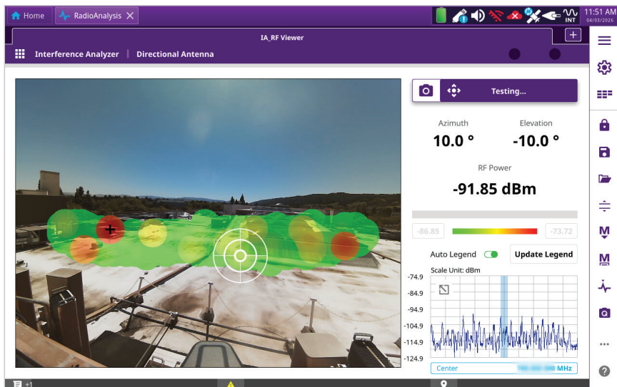
RF Viewer | PIM Generated Interference | Case 2 Sector Top E
