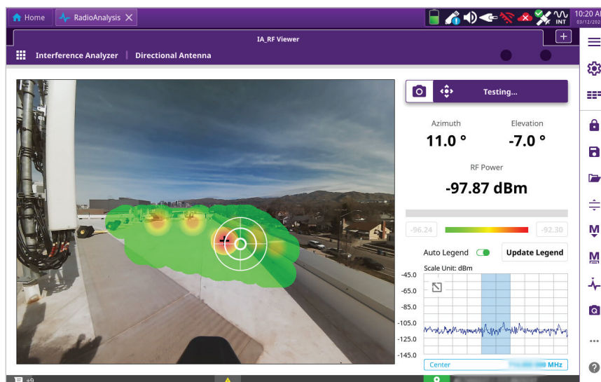
RF Viewer | PIM Generated Interference | Case 1 Sector Right
