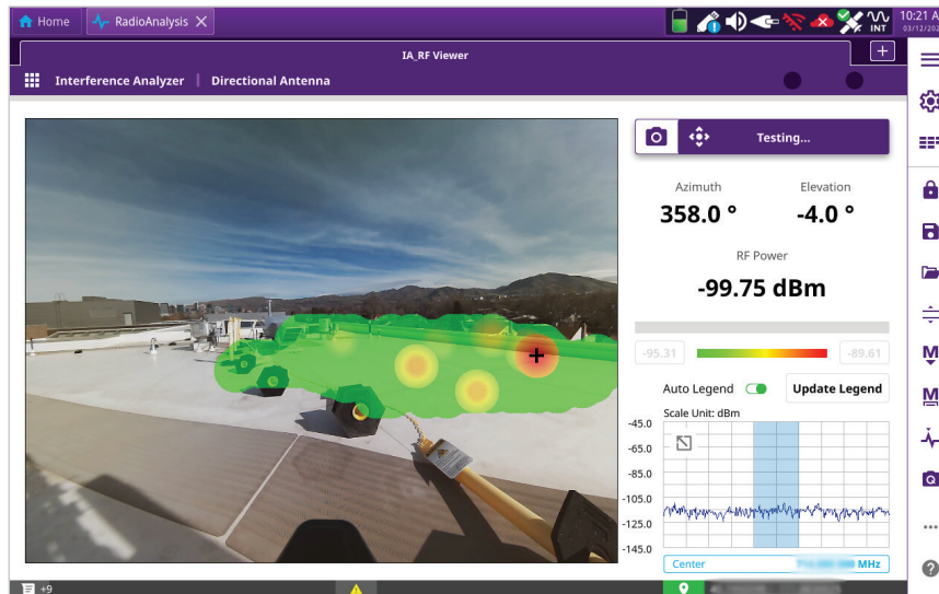
RF Viewer | PIM Generated Interference | Case 1 Sector Left
