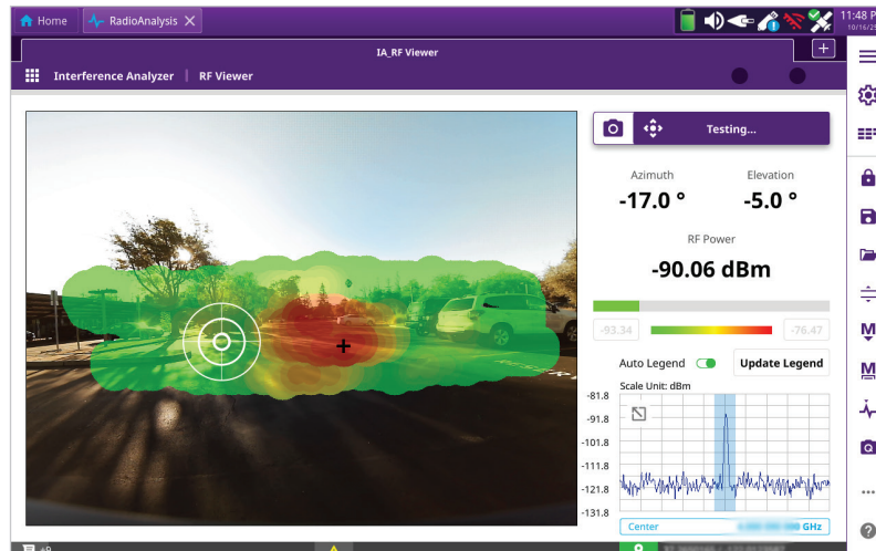
RF Viewer | Radiated External Interference | Case 1 at 386ft (118mts)
